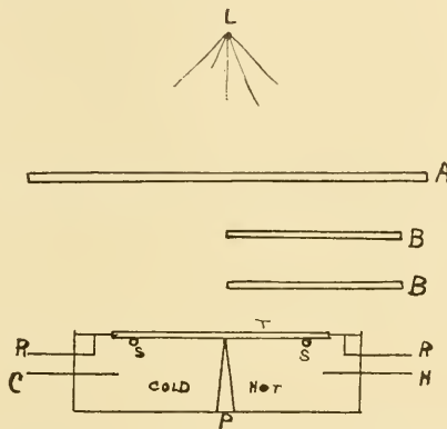
FIG. 4. A , alum bath heat screen. B B , light screens. C , cold water supply pipe. H , hot water supply pipe. L , electric light. P , Knife edge partition. R R , overflow return pipes. S S , supports for trough. T , trough.
